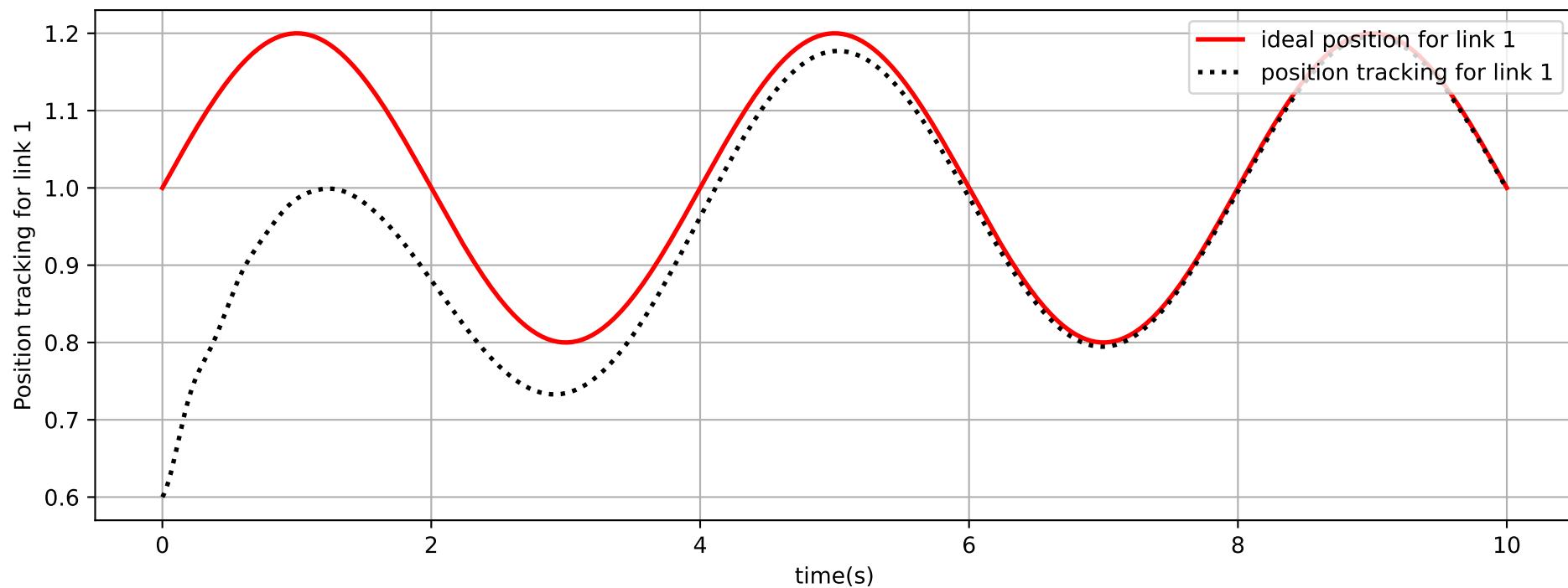
Position Tracking Performance ( S=3 , S1=2 , m=5 )
